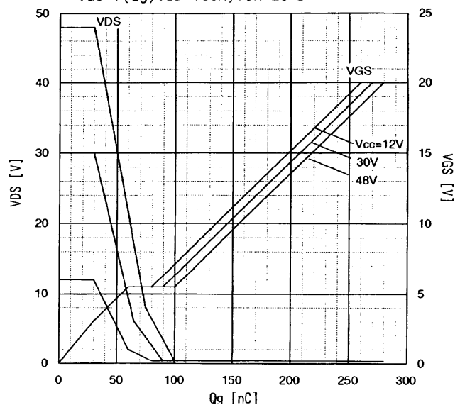
Typical Gate Charge Characteristics V_{GS} = f(Q_g) : I_D = 100A, Tch = 25°C
