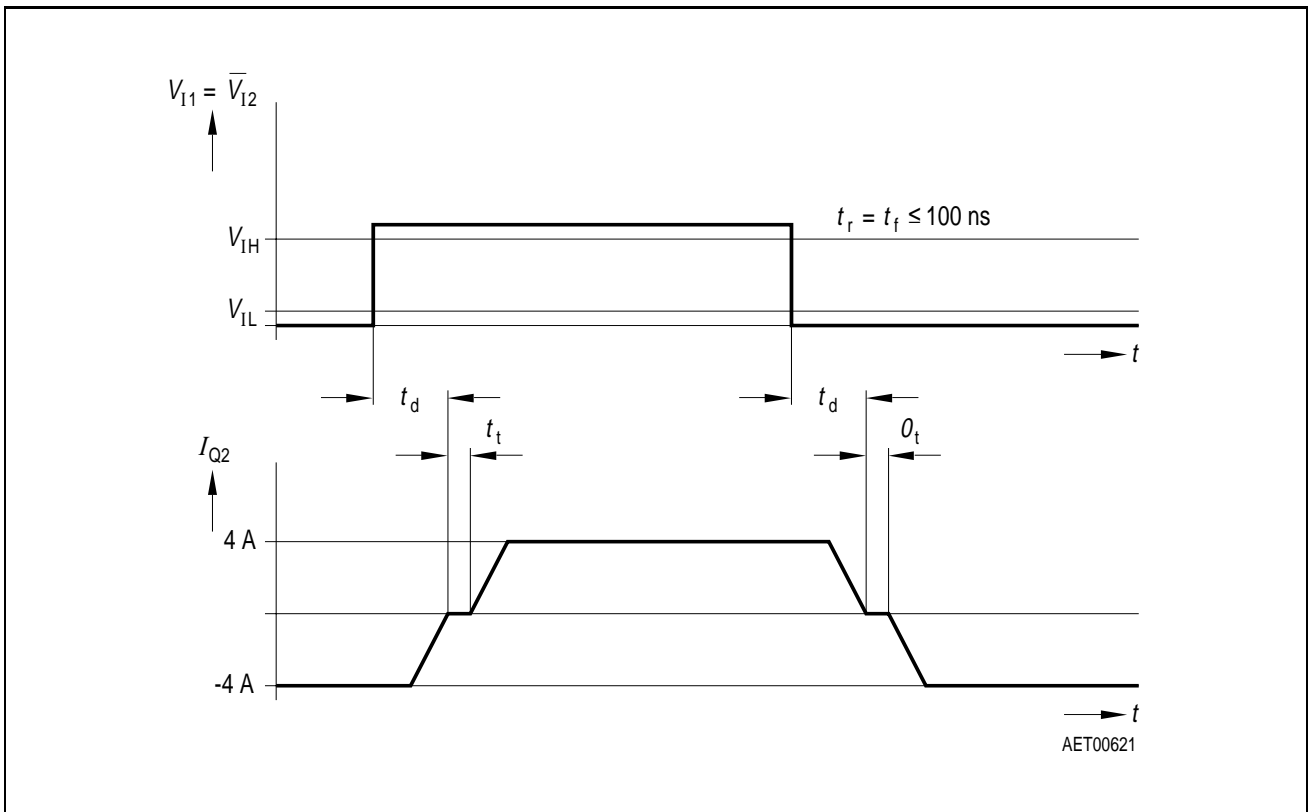
Figure 4 Timing Diagram
