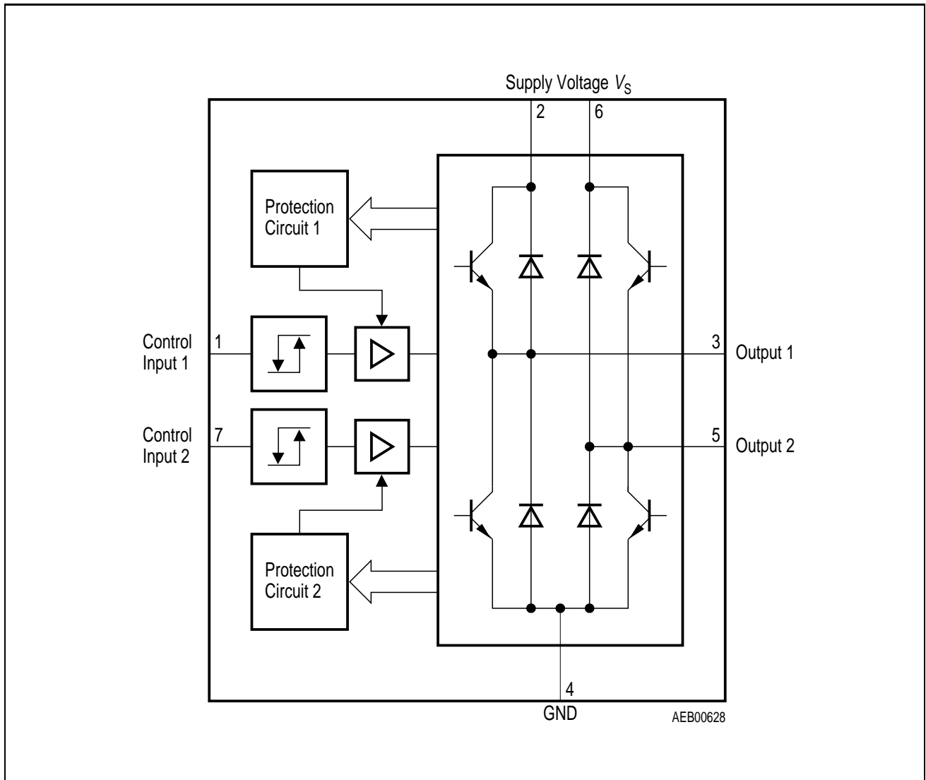
Figure 2 Block Diagram
