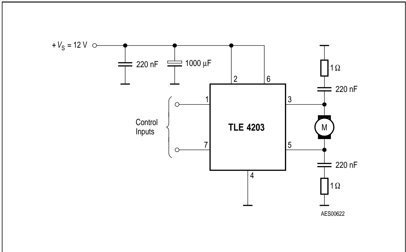
Figure 5 Application Circuit
